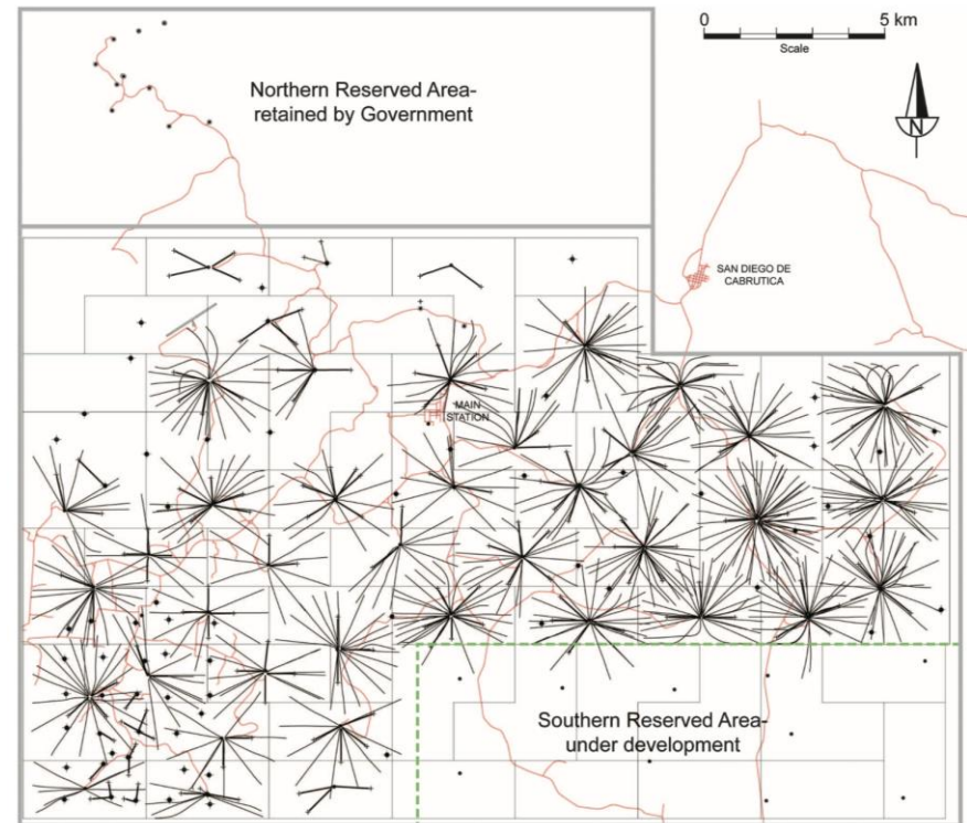
Sincor development scheme, radial horizontal wells
